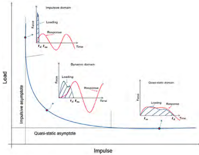
Figure 1. P-I diagram and load pulse domains [3].
