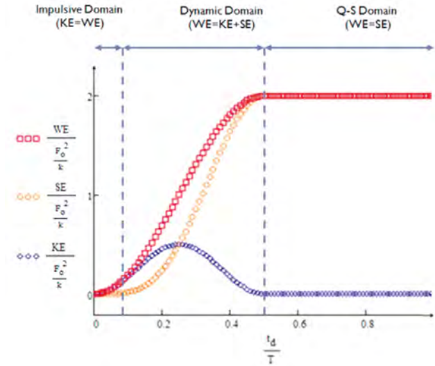
Figure 2. Typical energy components spectra [3].
