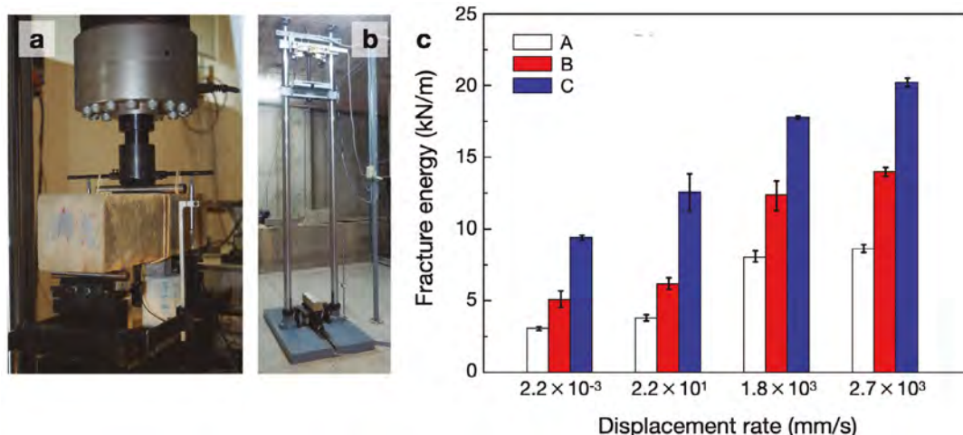
Figure 3. Fracture energy measurements at multiple displacement rates: (a) servo-hydraulic machine (2.2 \mu m/s and 22 mm/s); (b) drop-weight device (1.8 m/s and 2.7 m/s); (c) fracture energy vs. displacement rate for all mixes at \delta = 3 mm.
