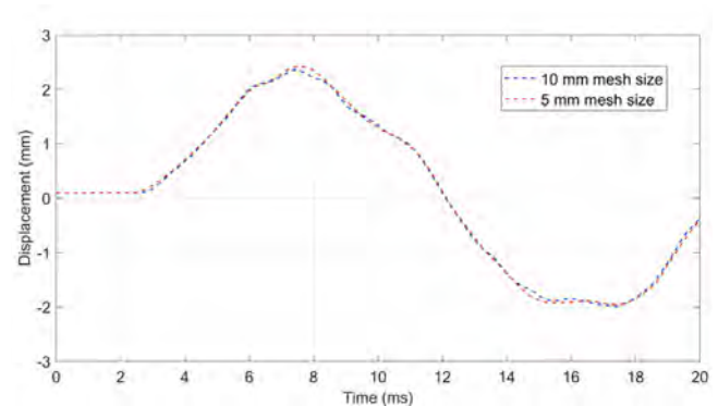
Figure 15. Result of displacement obtained in test E2/E3 for the mesh sensitivity test.
