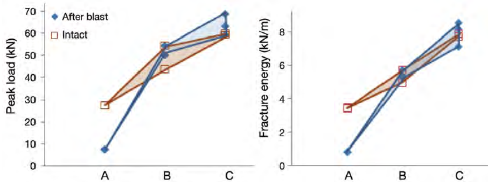
Figure 14. Comparison of the peak loads and fracture energies measured in the pristine and tested slabs for all concrete types.
