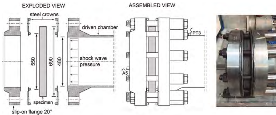
Figure 15. Details of the boundary conditions of the slab in the shock tube equipment (reprinted with the permission of the publisher – Colombo et al. 2021).
