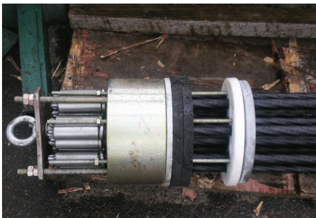
Figura 27. Nuevo anclaje superior con manguitos Figure 27. New top unions equipped with extrusion sleeves
