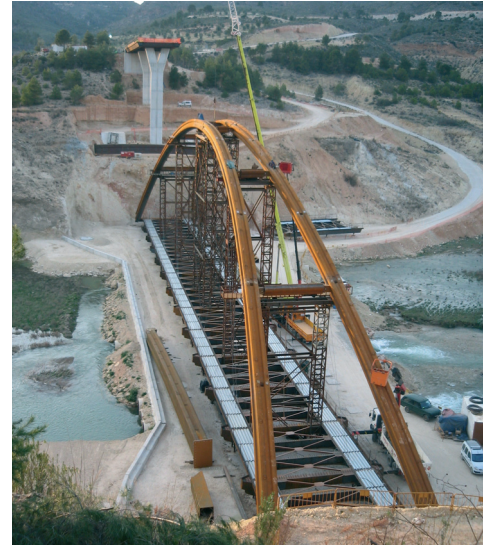
Figura 15. Bowstring (III). Desapeo y péndolas Figure 15. Bowstring (III). De-shoring and hangers
