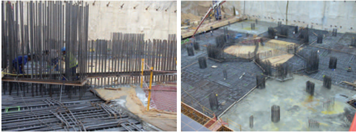
Figura 9. Plantilla de colocación de armado de núcleo y vista general del hormigonado de la segunda tongada de losa. Figure 9. Mould for the installation of the core reinforcement and general view of the concreting of the second concrete lift of the slab.
