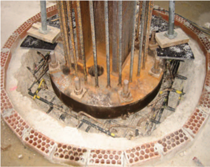
Figura 15. Detalle de la zona a hormigonar bajo placa. Figure 15. Detail of the area to be concreted under the plate.
